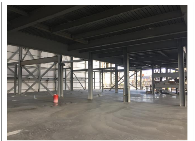
Concrete pours ongoing to auditoria level.
