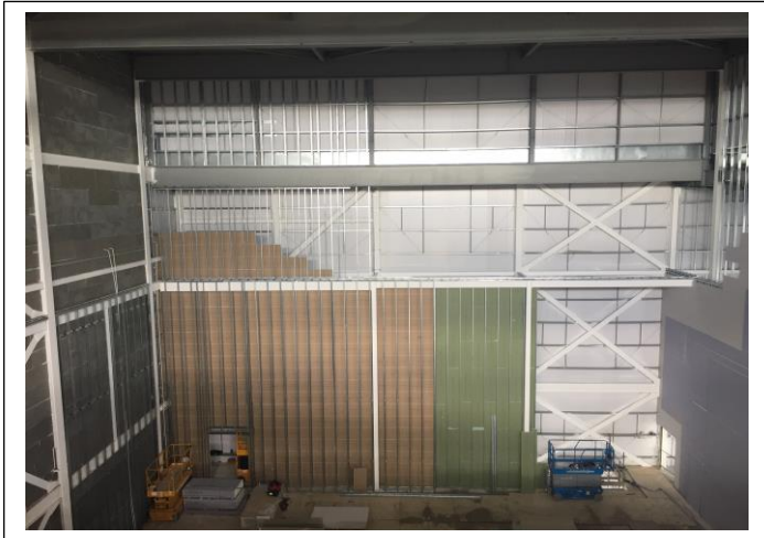
Dry lining ongoing to IMAX auditorium.
